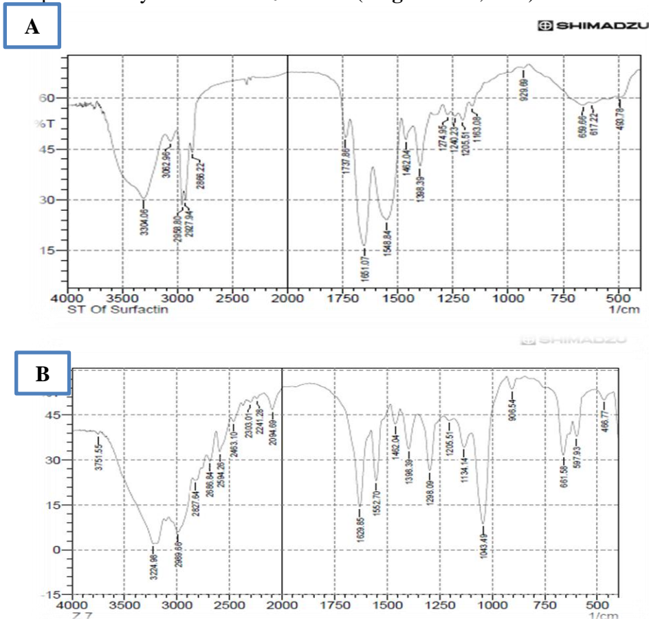
Figure (2): FTIR (A) spectrophotometer diagnosis of the standard surfactin and (B) lyophilized filtrate of B. subtilis ZE2013.
