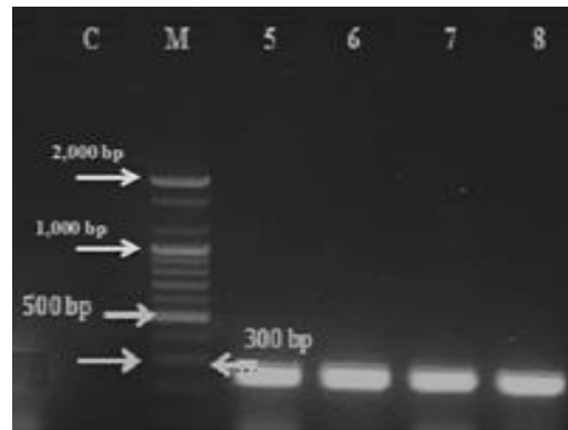
Figure (2): Electrophoresis of fungal isolates of S. sclerotiorum (isolate number 5-8) ~ 300 bp. PCR fragment.
